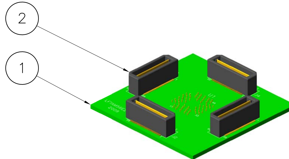
ISO PLAN VIEW
