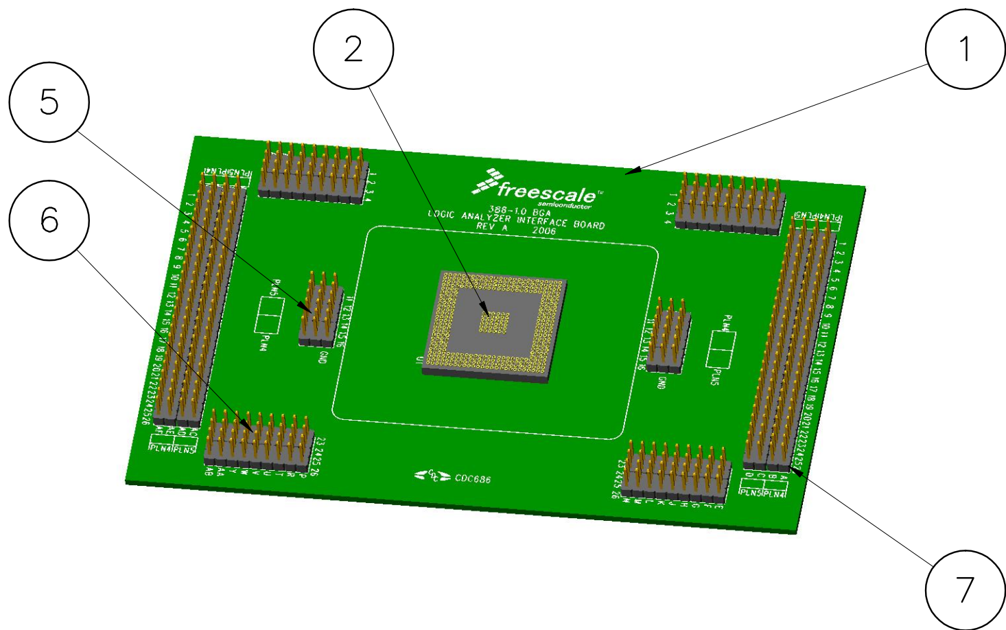
ISO TOP VIEW
